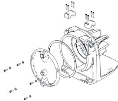
EP3 and EP4 Pump Module
