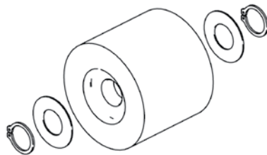
EP3 Roller Kit
